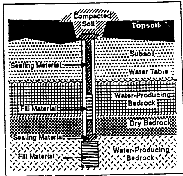
Figure 4. Recommended filling sequence for wells tapping more than one bedrock layer.
